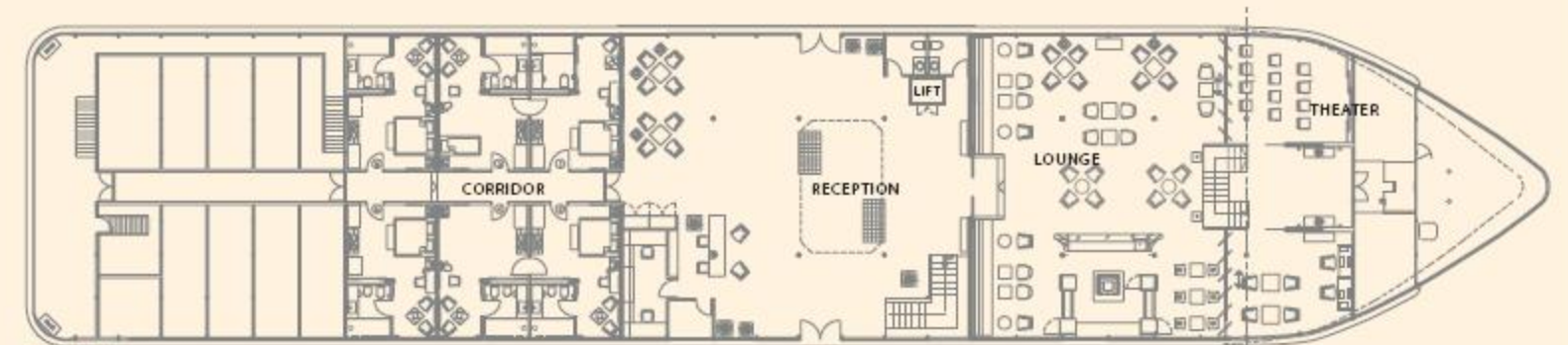
DECK - B
